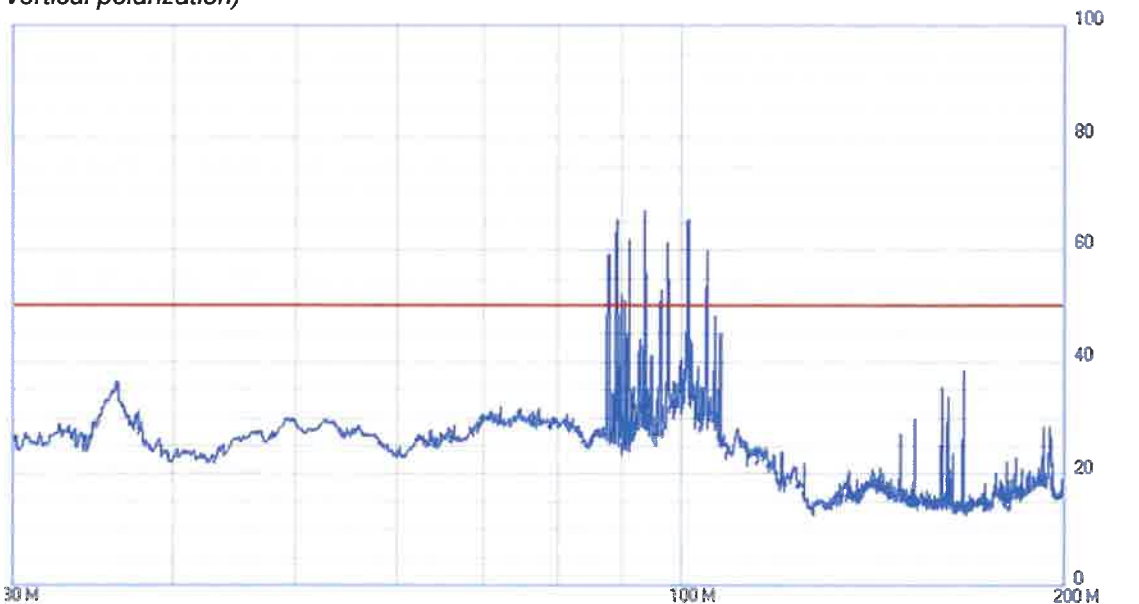
Graph 4 - Records of emissions from background – range 30 – 200 MHz - (envelope of horizontal and vertical polarization)
